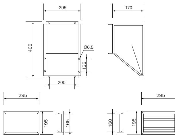
Fig 2. Mixing cabinet (accessory)
